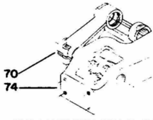
VIEW SHOWING N° 70 ARBOR BRACKET AND N° 74 YOKE ASSEMBLED.
